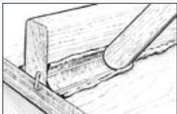
Figure 13 Shape and smooth the fillet.
