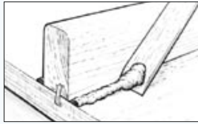
Figure 12 Remove or shape excess epoxy that squeezes out of the joint.
